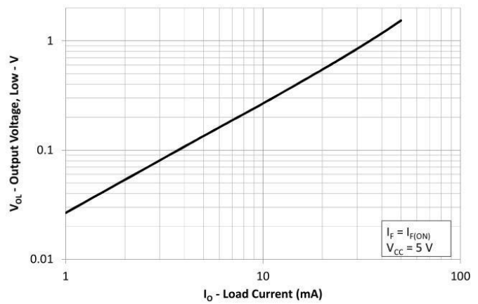
Figure 4. Output Voltage, Low vs. Load Current
