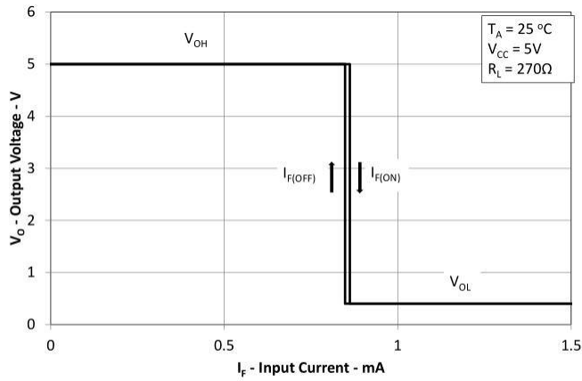
Figure 1. Transfer Characteristic
