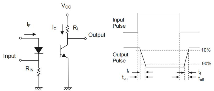
Fig.14 Switching Time Test Circuit & Waveforms
