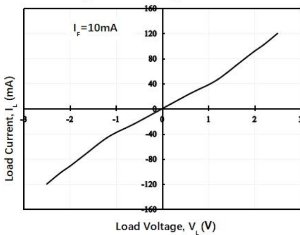
Figure 7. Load Voltage VS Load Current
