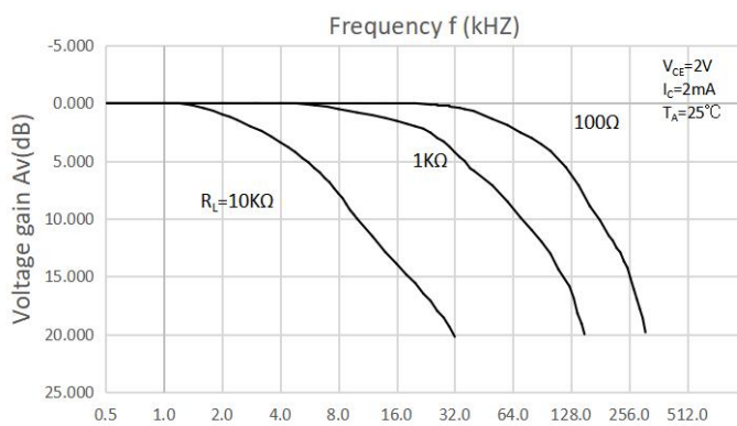
Fig.11 Frequency Response
